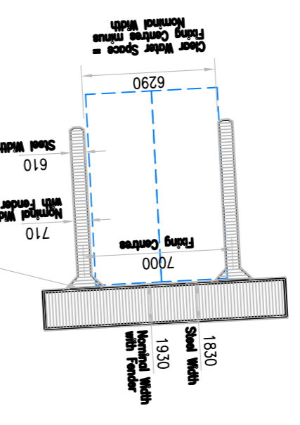
9m x 3.1m Berth showing pontoon dimensions
